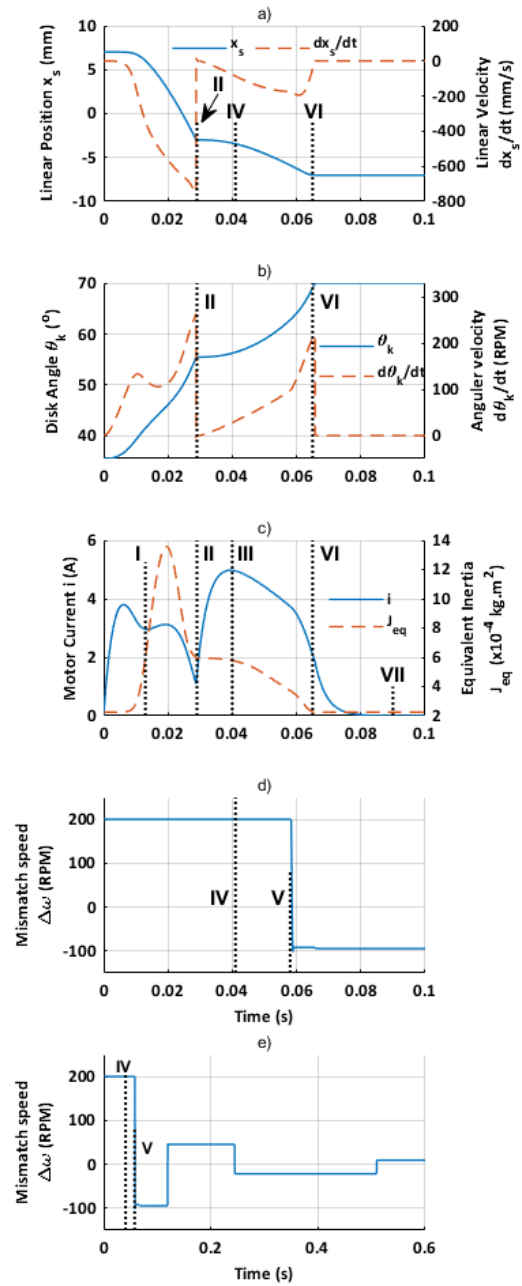
Figure 11. 1 st to 2 nd gear shift open-loop response for a) sleeve's linear position and speed, b) disk angle and angular speed, c) motor current and equivalent inertia, and d) Mismatch speed. Key time points: I: 0.013 s, II: 0.029 s, III: 0.04 s, IV: 0.041 s, V: 0.058 s, VI: 0.065 s and VII: 0.09 s.
