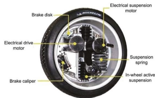
Figure 6: Michelin Active Wheel, (Jandura, Břoušek and Bukvic, 2015).
