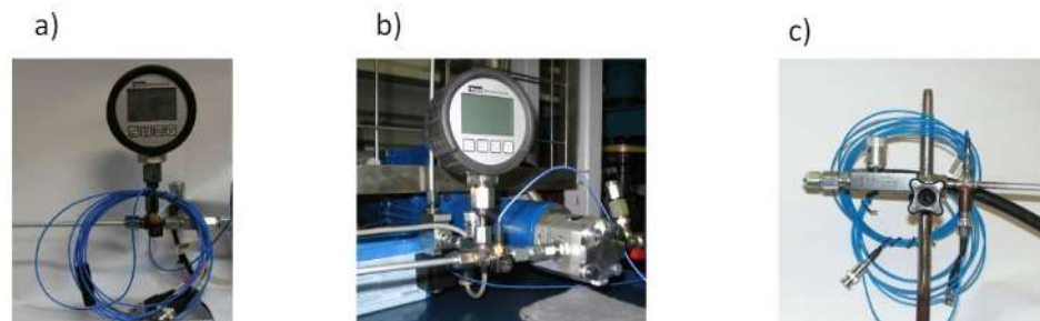
Figure 4. Point of measurement for the acceleration of mechanical vibrations of the hydraulic microtube and pressure pulsation in the microhydraulic system: a), b) at the micropump, c) at the throttle microvalve
